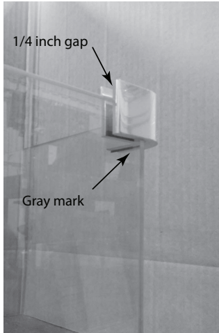
Figure 3 Align Marks
